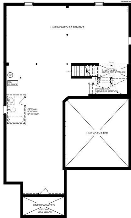
BASEMENT ELEVATION A & B
